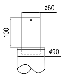
SPIGOT DETAIL
