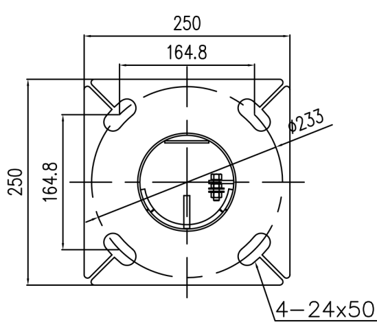
BASEPLATE FOR 4-M20@233PCD RAGBOLTS
