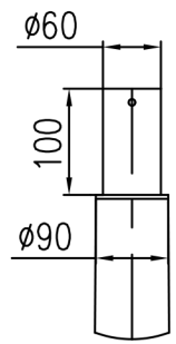
SPIGOT DETAIL
