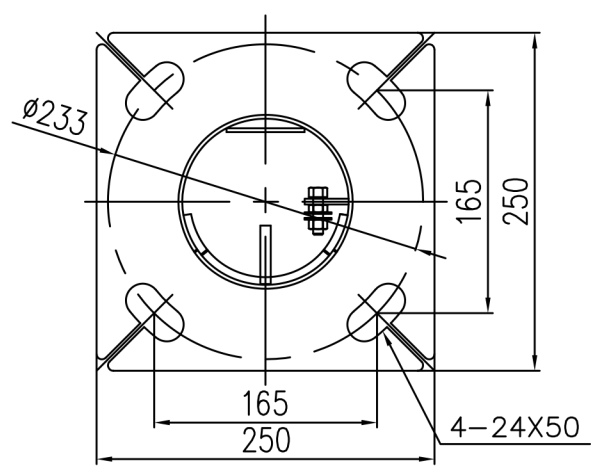
BASEPLATE FOR 4-M20@233 PCD RAGBOLTS
